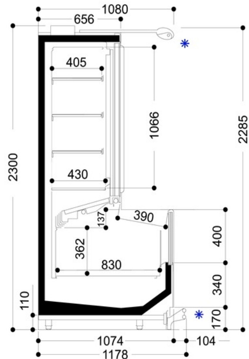
MIURA H2200 - HG400
