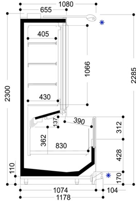
MIURA H2200 - LG300
