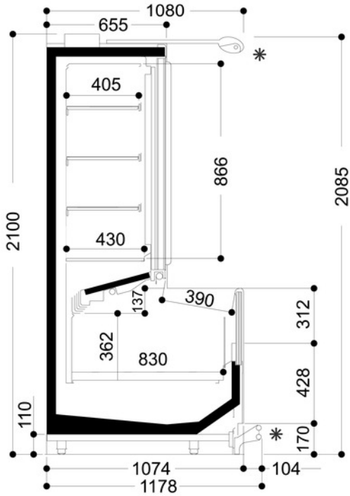
MIURA H2000 - LG300
