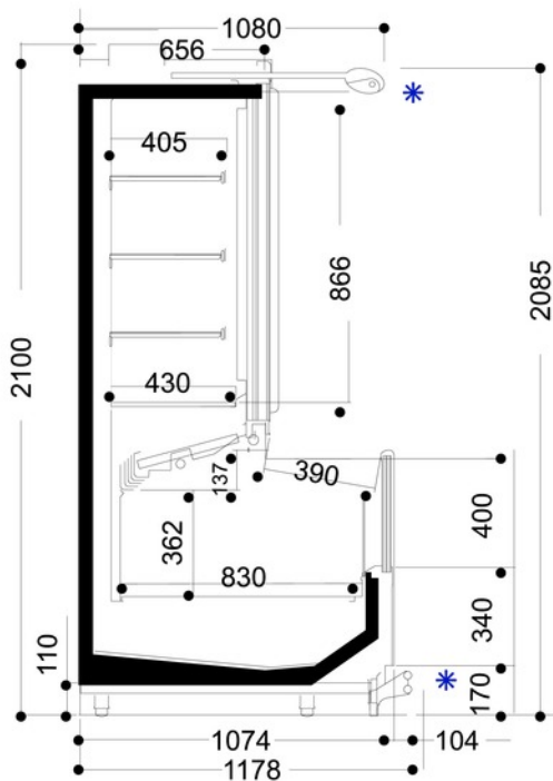
MIURA H2000 - HG400
